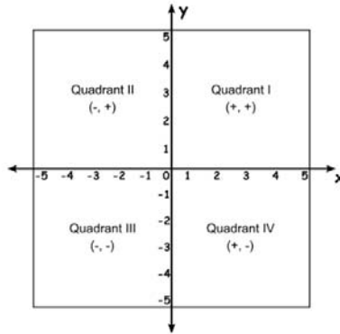
Figure of the quadrants of coordinate plane.
